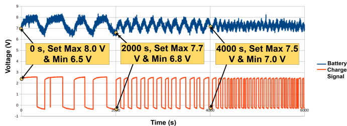
Fig. 3. Maintenance of three battery voltage ranges by the PCS
