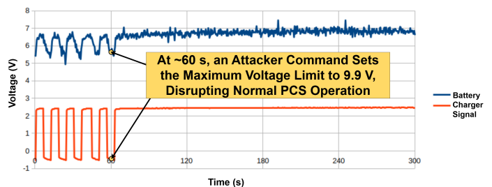
Fig. 5. Failure of battery maintenance after unauthorized command attack.
