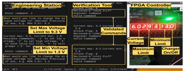
Fig. 4. Normal operation of the PCS experimental testbed.
