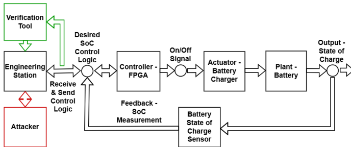
Fig. 1. Control Loop Block Diagram for Battery Charging Process Control System. Components within the main control loop are colored black, whereas external components that communicate with the control system are depicted in color. The legitimate external sources of communication in this diagram are represented with green arrows, whereas adversary sources are represented with red arrows.
