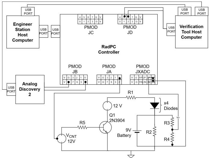
Fig. 2. Wired Connections of the process control system (PCS).
