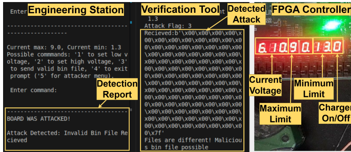
Fig. 6. Detection & mitigation of malicious firmware upload.
