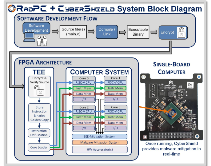
Fig. 2: System block diagram of RadPC + TEE i.e. Cybershield. Illustrates the software development flow, FPGA architecture, and the single-board computer.
