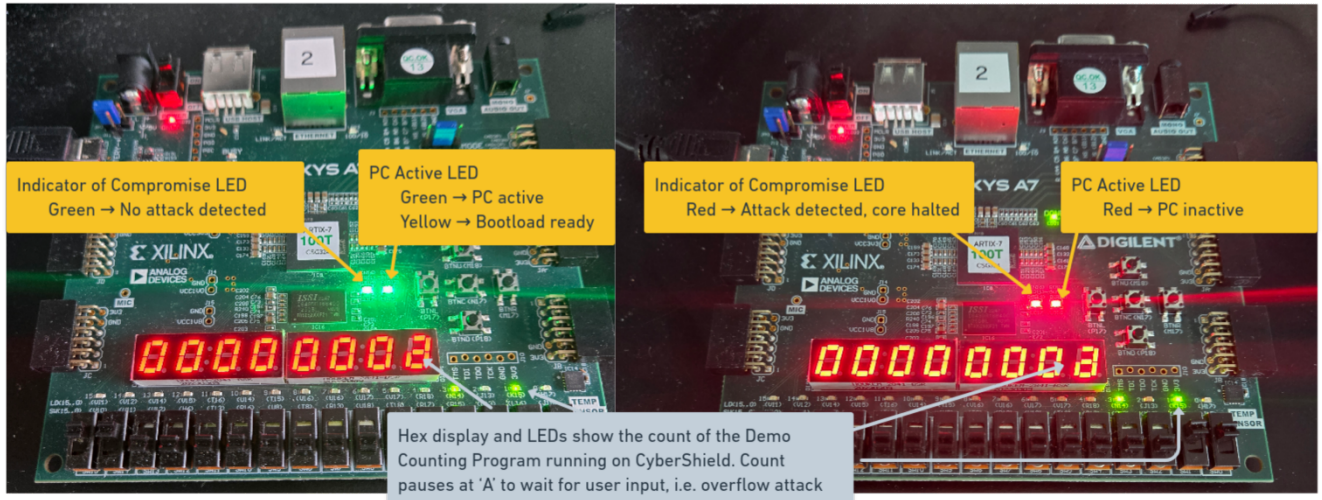
Fig. 6: Two Nexys A7 boards demonstrating CyberShield’s runtime behavior. Left board: The green LED on the left indicates that CyberShield has booted successfully and no indicator of compromise (IoC) has been detected. The green LED on the right functions as a PC active flag, signifying that the cores are currently executing instructions normally. Right board: In contrast, the left red LED indicates that an IoC has been detected, signaling that the system has identified an attack. The right red LED, which normally serves as the PC active flag, now indicates that all cores have been halted to prevent further execution of potentially malicious instructions.
