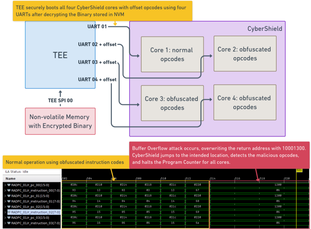
Fig. 5: Diagram of the CyberShield architecture with CyberShield and TEE integration, accompanied by ILA outputs. The diagram illustrates how the TEE securely bootloads each CyberShield core with its assigned opcode offset: Core 1 executes standard RISC-V opcodes, while Cores 2–4 operate with unique, offset opcodes. The ILA shows the cores running offset opcodes during normal operation. When a buffer overflow attack occurs, all four cores are forced to execute identical opcodes. The anti-voter in CyberShield detects that all four cores are running the same opcode and freezes the program counter to prevent the cores from executing the malicious code.
