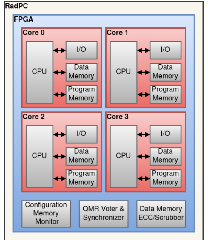
Fig. 1: Block diagram of the QMR architecture of the RadPC FPGA system [12].
